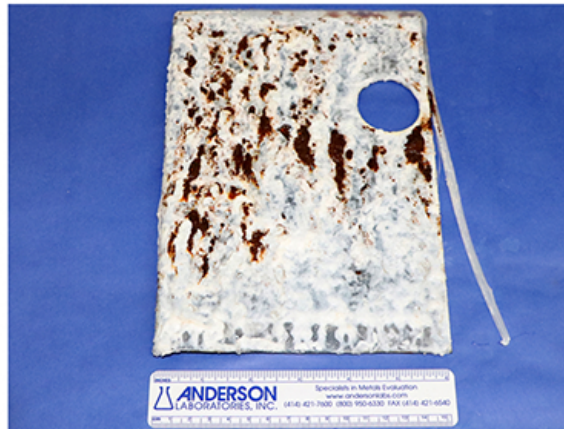
G235 Flat w/Perf.
