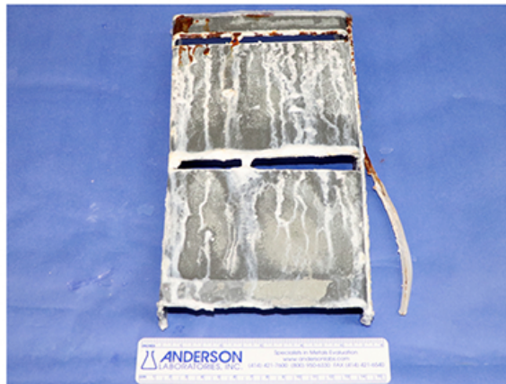
HDG G40 + CG-AG Expanded Sidewall - Edge Test
