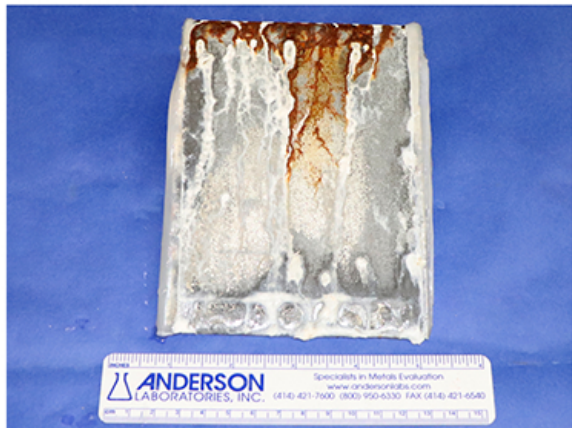
HDG G40 + CG-AG Overbend (Tool Defects)
